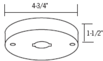
Mono-Point Adapters
